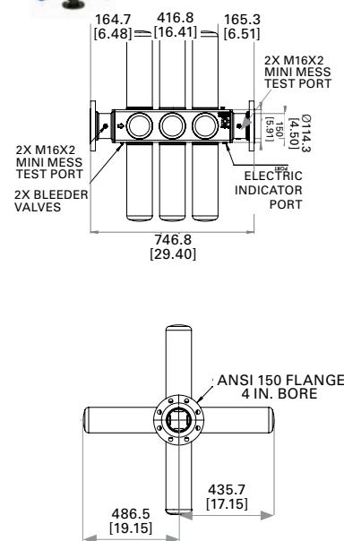
Inline 12 Manifold 1KDF1012
