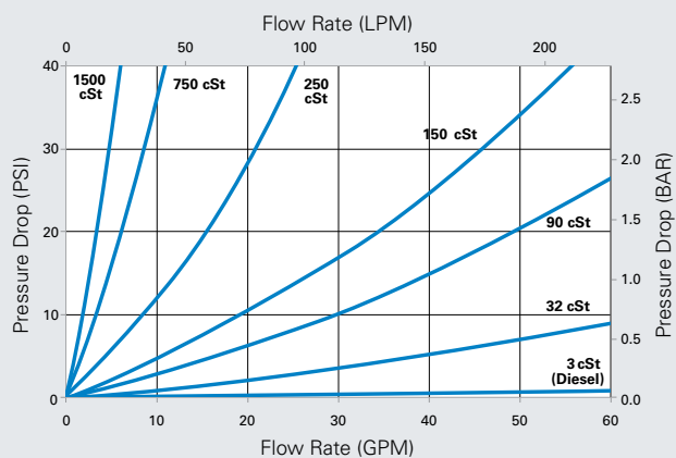
DBB8777 - Winter Fuel Filter
