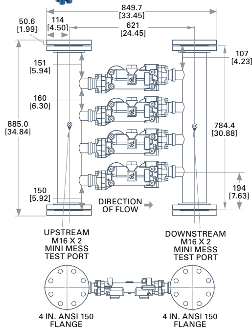
8 Filter Manifold P568932
