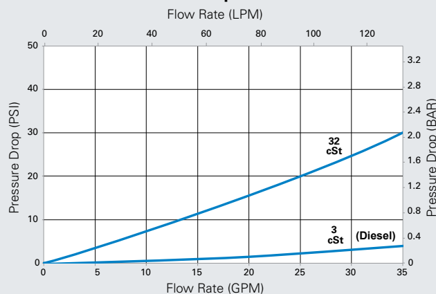
DBB5333 - Compact Fuel Filter
