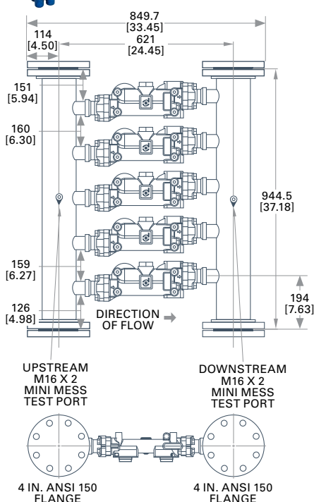
10 Filter Manifold P568933
