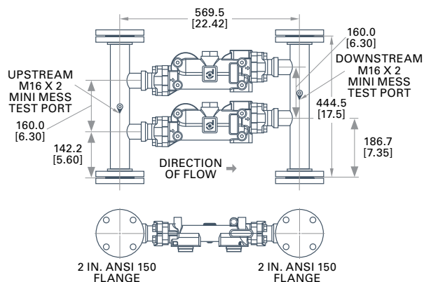
4 Filter Manifold P561880
