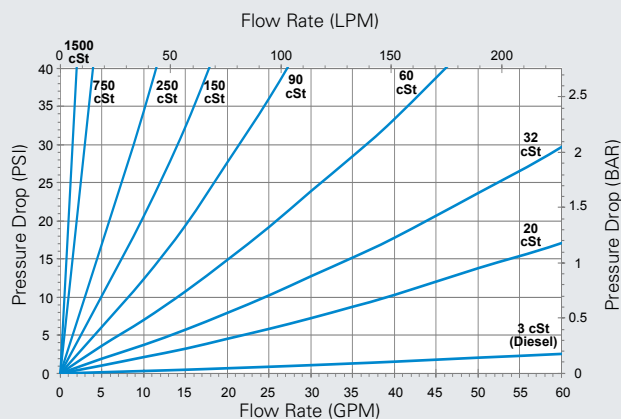
DBB8666 - Fuel Filter
