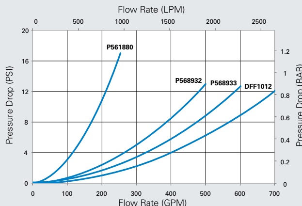
Manifold Pressure Drop
