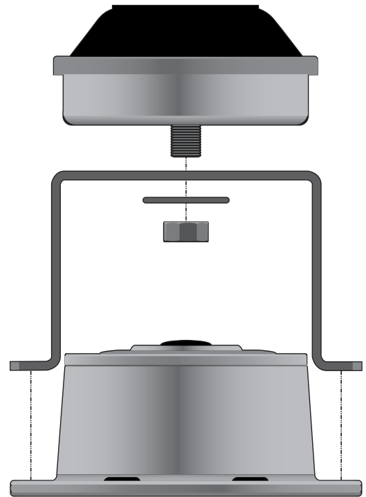
Hubodometer Mount
